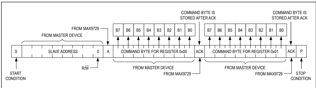
Figure 6b. Write Data Format for Writing to Registers 0x00 and 0x01
