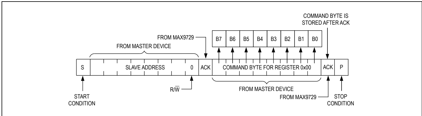
Figure 6a. Write Data Format for Writing to Register 0x00 Only
