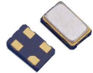
Part Dimensions: 5.0 × 3.2 × 1.3mm • 60.7734mg
