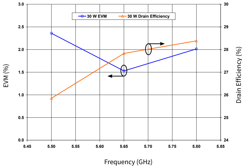
Figure 2. Typical EVM and Efficiency vs Frequency of CGH55030F1 and CGH55030P1 in the CGH55030-AMP V_{DD} = 28\text{ V}, I_{DQ} = 250\text{ mA}, 802.16\text{-}2004\text{ OFDM}, PAR = 9.8\text{ dB}, P_{AVE} = 5\text{ W}
