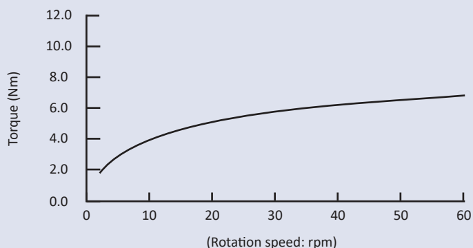
Speed characteristics of FDN-63A-453 series (Measurement temperature: 23°C)
