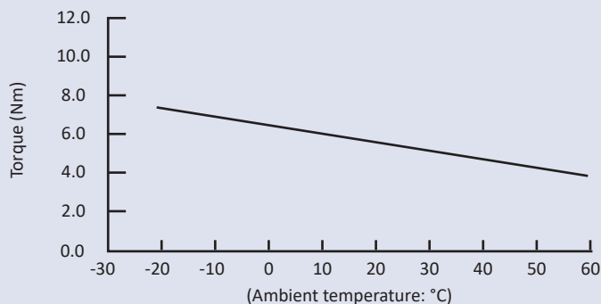
Temperature characteristics of FDN-63A-453 series (Rotation speed: 20 rpm)
