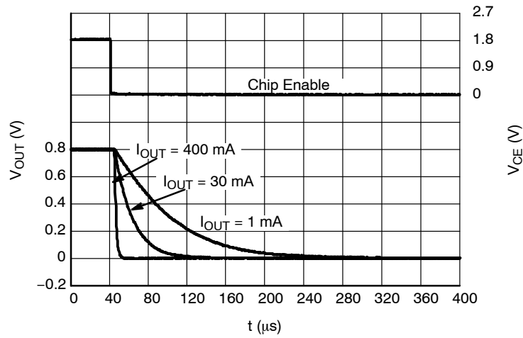
Figure 42. Shutdown, 0.8 V Version, V_{IN} = 1.8 V
