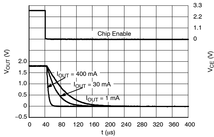
Figure 44. Shutdown, 1.8 V Version, V_{IN} = 2.8 V
