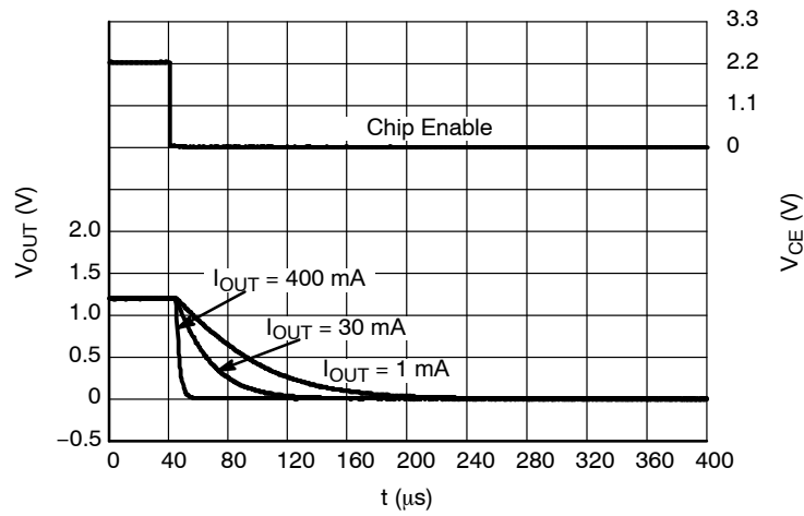
Figure 43. Shutdown, 1.2 V Version, V_{IN} = 2.2 V
