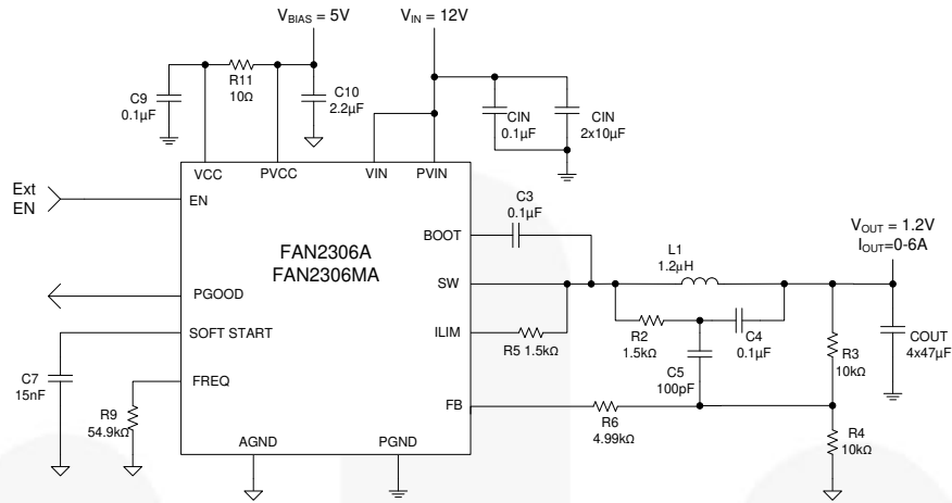
Figure 1. Typical Application
