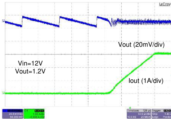
Figure 17. FAN2306MA Transition from DCM to CCM
