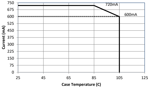
Figure 8: Derating Curve
