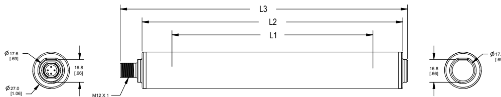
Figure 2. Cascade Models
