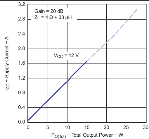
Note: Dashed Lines represent thermally limited regions. Figure 26. Supply Current vs Total Output Power (BTL)
