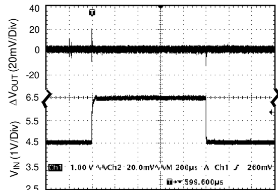
Time (200µs/Div)
