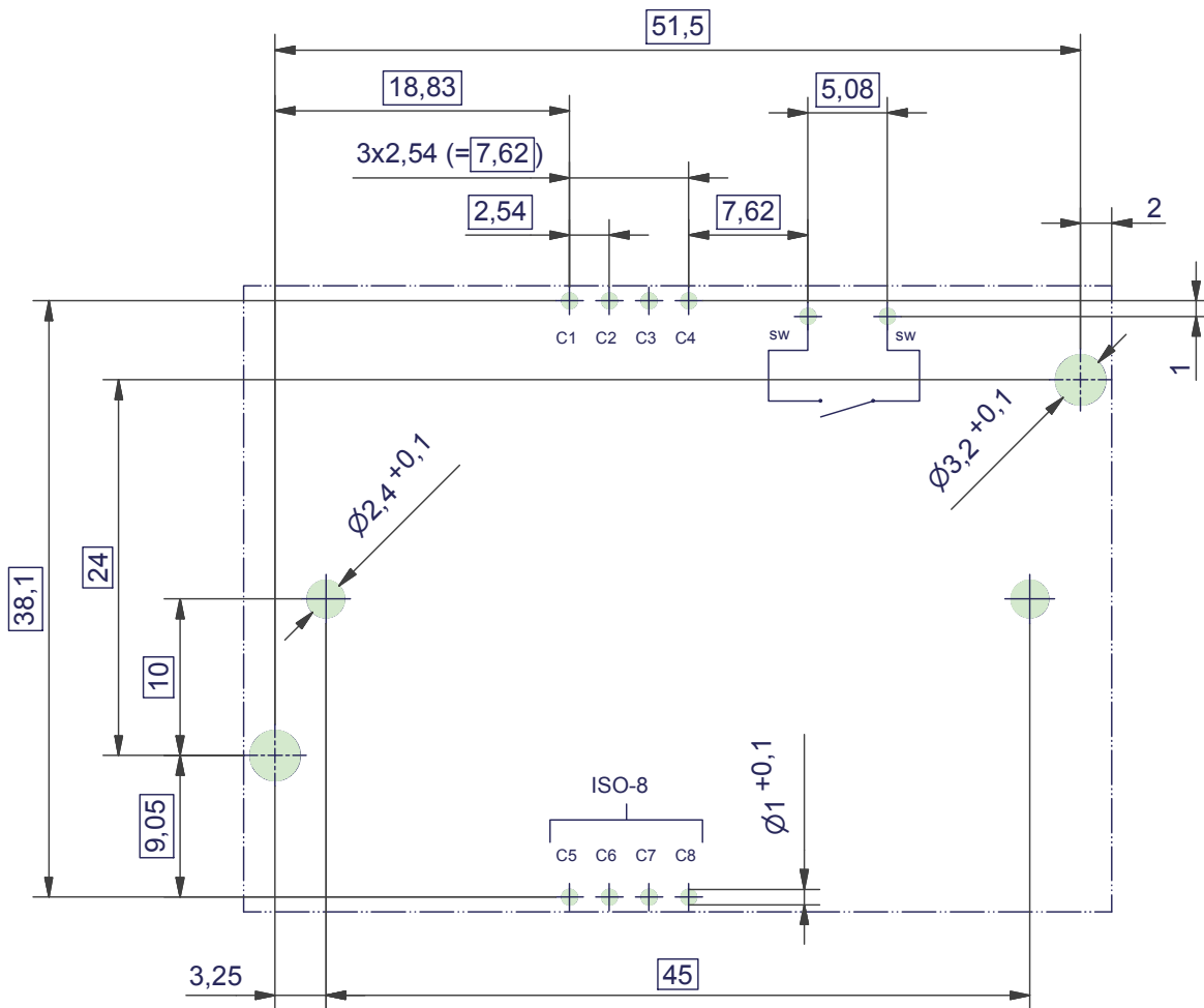
Drilling matrix (Component side)
