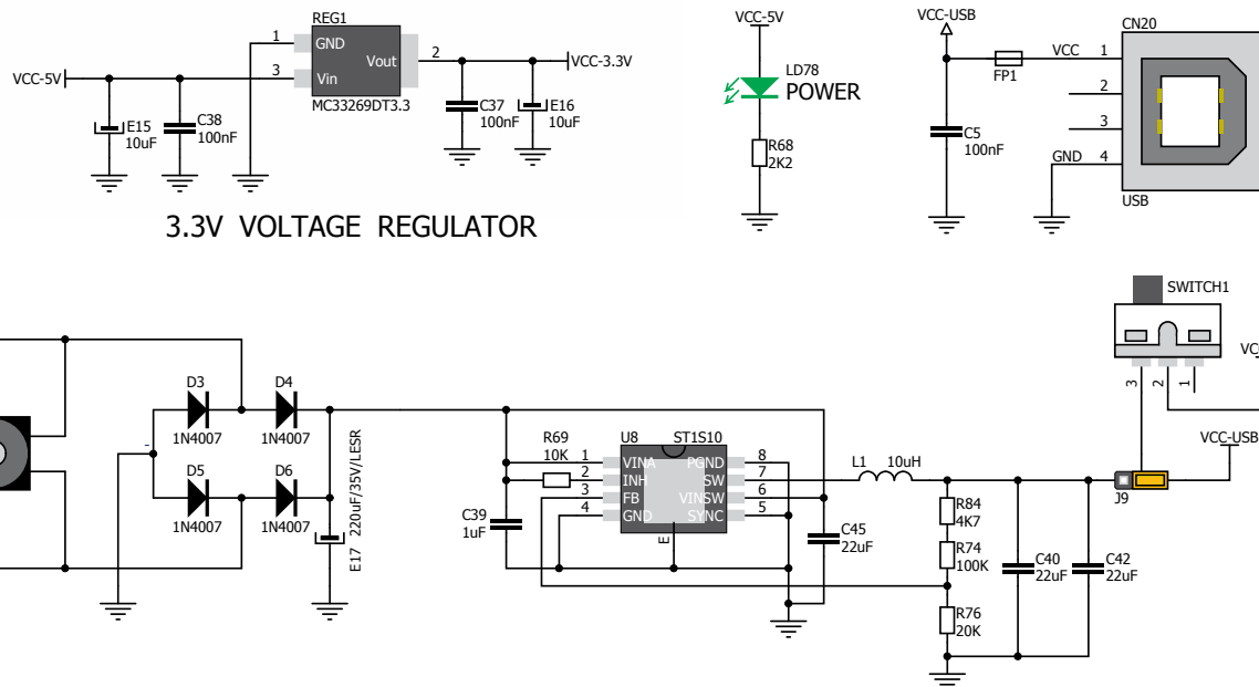
Figure 3-2: Power supply unit schematic
