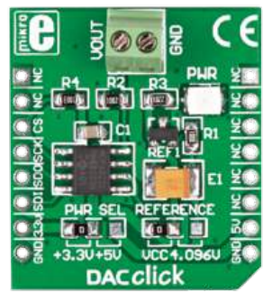
DAC click™
