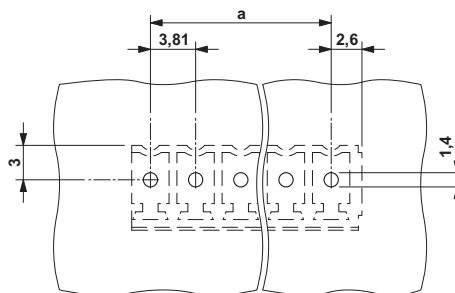
Drilling diagram
