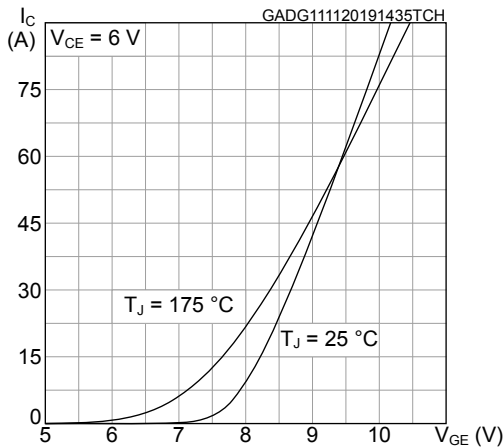
Figure 9. Transfer characteristics
