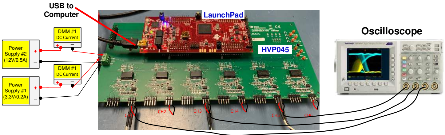
Figure 3-1. Bench Setup Configuration
