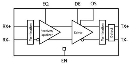
Figure 1. Logic Diagram of NB7VPQ701M
