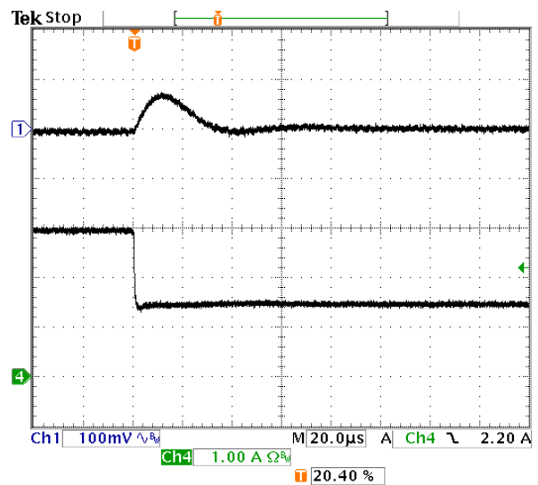
Fig-1.0V-7: Output voltage response for V_{out}=1.0V to negative load current step change from 3A to 1.5A with slew rate of -5A/\mu s at V_{in}=12V . C_o=47\mu F \times 2 ceramic. Top trace: output voltage (100mV/div.) Bottom trace: load current (1A/div.) Time scale: 20us/div.
