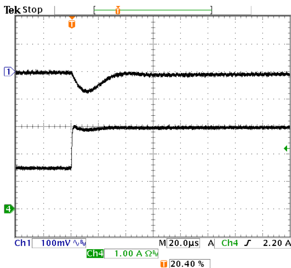
Fig-1.0V-6: Output voltage response for V_{out}=1.0V to positive load current step change from 1.5A to 3A with slew rate of 5A/\mu s at V_{in}=12V . C_o=47\mu F \times 2 ceramic. Top trace: output voltage (100mV/div.) Bottom trace: load current (1A/div.) Time scale: 20us/div.
