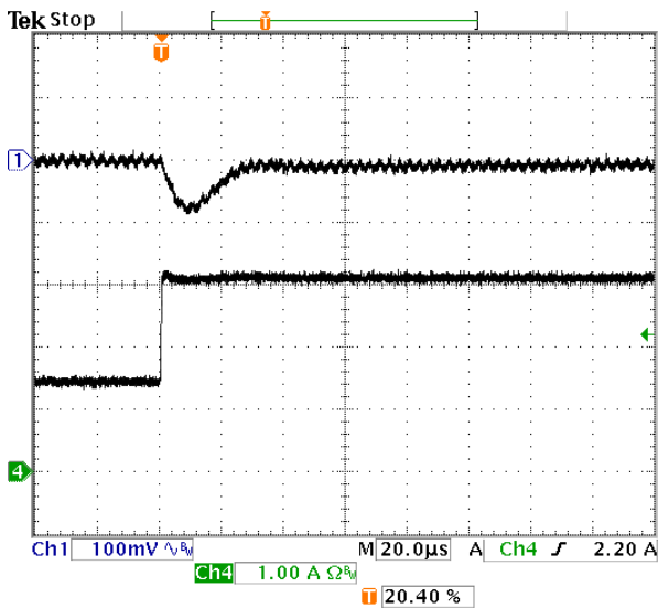
Fig-3.3V-6: Output voltage response for V_{out}=3.3V to positive load current step change from 1.5A to 3A with slew rate of 5A/us at V_{in}=12V . C_o=47\mu F \times 2 ceramic. Top trace: output voltage (100mV/div.) Bottom trace: load current (1A/div.) Time scale: 20us/div.
