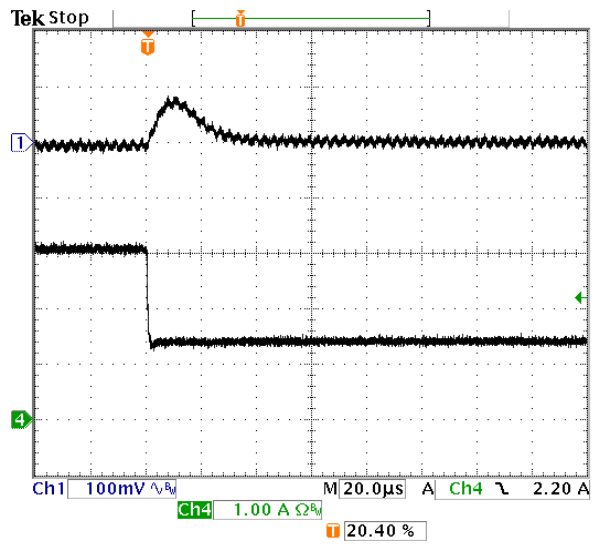
Fig-3.3V-7: Output voltage response for V_{out}=3.3V to negative load current step change from 3A to 1.5A with slew rate of -5A/us at V_{in}=12V . C_o=47\mu F \times 2 ceramic. Top trace: output voltage (100mV/div.) Bottom trace: load current (1A/div.) Time scale: 20us/div.
