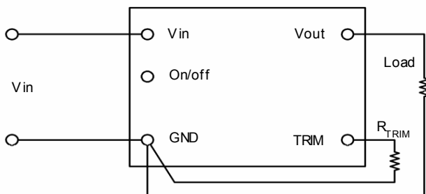
Fig. B: Configuration for programming output voltage
