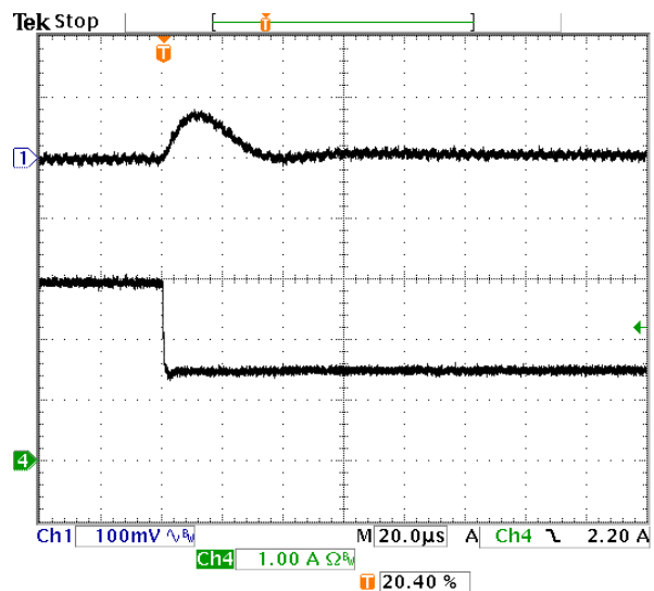
Fig-1.8V-7: Output voltage response for V_{out}=1.8V to negative load current step change from 3A to 1.5A with slew rate of -5A/\mu s at V_{in}=12V . C_o=47\mu F \times 2 ceramic. Top trace: output voltage (100mV/div.) Bottom trace: load current (1A/div.) Time scale: 20us/div.
