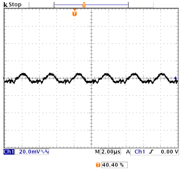
Fig-3.3V-5: Output voltage ripple (20mV/div.) for V_{out}=3.3V at full rated load current into a resistive load with external capacitance 47\mu F \times 2 ceramic + 1uF ceramic at V_{in}=12V . Time scale: 2 us/div.
