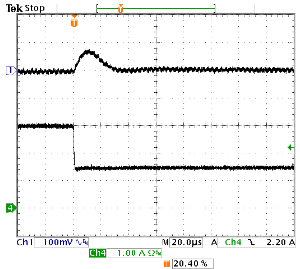
Fig-2.5V-7: Output voltage response for V_{out}=2.5V to negative load current step change from 3A to 1.5A with slew rate of -5A/\mu s at V_{in}=12V . C_o=47\mu F \times 2 ceramic.
