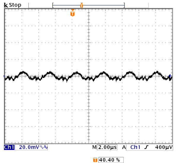
Fig-2.5V-5: Output voltage ripple (20mV/div.) for V_{out}=2.5V at full rated load current into a resistive load with external capacitance 47\mu F \times 2 ceramic + 1\mu F ceramic at V_{in}=12V .
