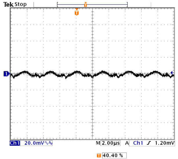
Fig-1.2V-5: Output voltage ripple (20mV/div.) for V_{out}=1.2V at full rated load current into a resistive load with external capacitance 47\mu F \times 2 ceramic + 1\mu F ceramic at V_{in}=12V .
