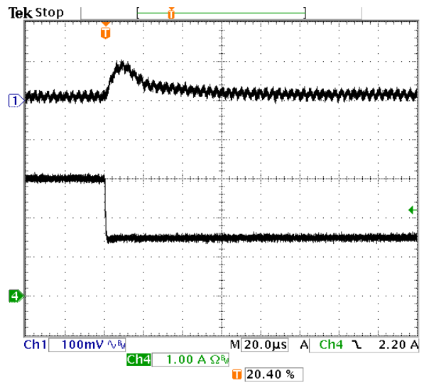
Fig-5.0V-7: Output voltage response for V_{out}=5.0V to negative load current step change from 3A to 1.5A with slew rate of -5A/\mu s at V_{in}=12V . C_o=47\mu F \times 2 ceramic. Top trace: output voltage (100mV/div.) Bottom trace: load current (1A/div.) Time scale: 20us/div.
