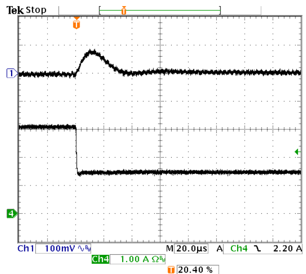
Fig-2.0V-7: Output voltage response for V_{out}=2.0V to negative load current step change from 3A to 1.5A with slew rate of -5A/us at V_{in}=12.0V . C_o=47\mu F \times 2 ceramic. Top trace: output voltage (100mV/div.) Bottom trace: load current (1A/div.) Time scale: 20us/div.
