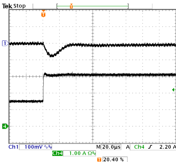
Fig-2.0V-6: Output voltage response for V_{out}=2.0V to positive load current step change from 1.5A to 3A with slew rate of 5A/us at V_{in}=12V . C_o=47\mu F \times 2 ceramic. Top trace: output voltage (100mV/div.) Bottom trace: load current (1A/div.) Time scale: 20us/div.
