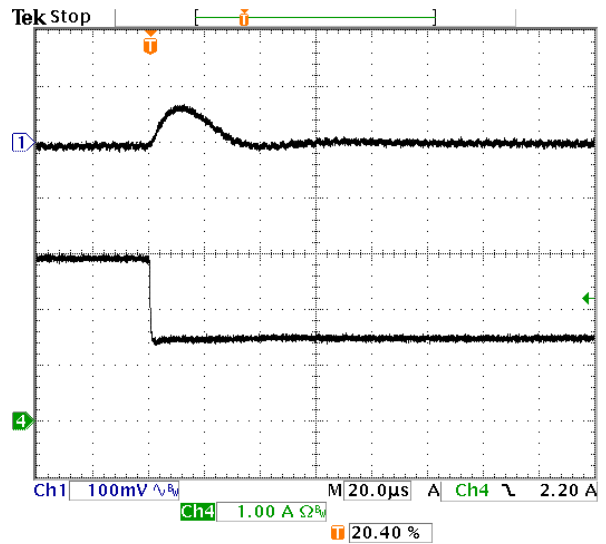
Fig-1.2V-7: Output voltage response for V_{out}=1.2V to negative load current step change from 3A to 1.5A with slew rate of -5A/\mu s at V_{in}=12V . C_o=47\mu F \times 2 ceramic.
