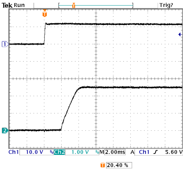
Fig-2.5V-4: Turn-on transient for V_{out}=2.5V with application of V_{in} at full rated load current (resistive) and 47\mu F \times 2 external capacitance at V_{in}=12V .
