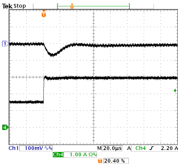
Fig-1.8V-6: Output voltage response for V_{out}=1.8V to positive load current step change from 1.5A to 3A with slew rate of 5A/\mu s at V_{in}=12V . C_o=47\mu F \times 2 ceramic. Top trace: output voltage (100mV/div.) Bottom trace: load current (1A/div.) Time scale: 20us/div.
