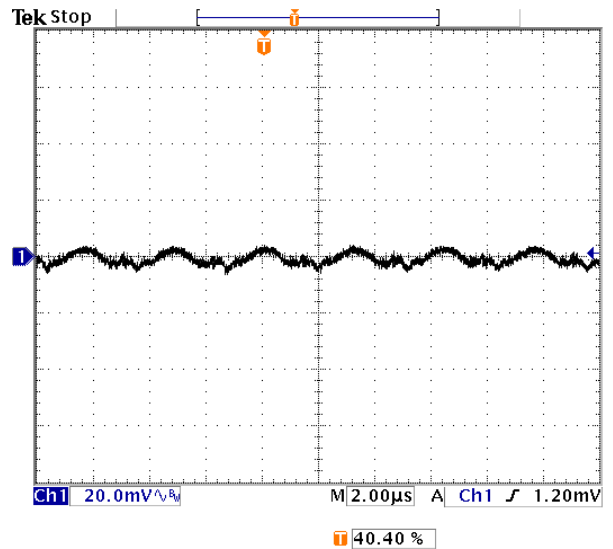
Fig-1.5V-5: Output voltage ripple (20mV/div.) for V_{out}=1.5V at full rated load current into a resistive load with external capacitance 47\mu F \times 2 ceramic + 1uF ceramic at V_{in}=12V . Time scale: 2 us/div
