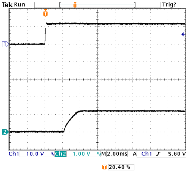
Fig-1.2V-4: Turn-on transient for V_{out}=1.2V with application of V_{in} at full rated load current (resistive) and 47\mu F \times 2 external capacitance at V_{in}=12V .
