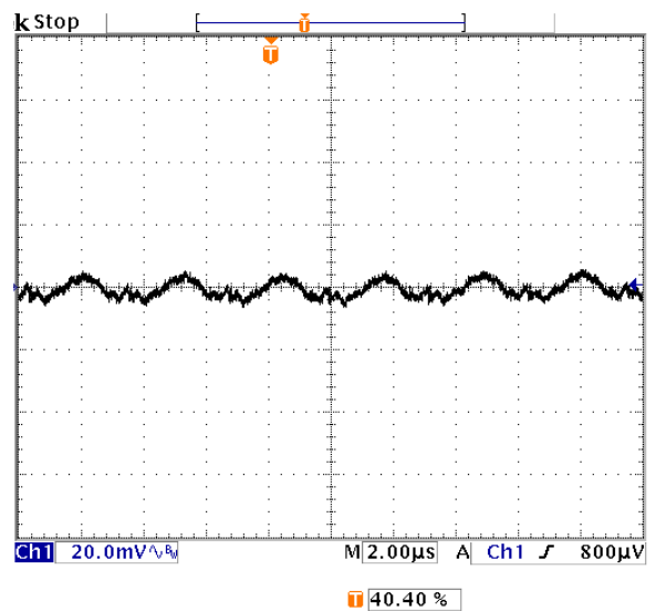
Fig-2.0V-5: Output voltage ripple (20mV/div.) for V_{out}=2.0V at full rated load current into a resistive load with external capacitance 47\mu F \times 2 ceramic + 1uF ceramic at V_{in}=12V . Time scale: 2 us/div.
