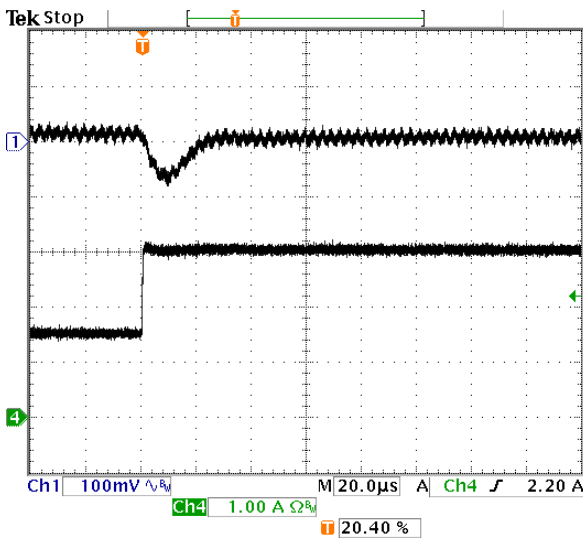
Fig-5.0V-6: Output voltage response for V_{out}=5.0V to positive load current step change from 1.5A to 3A with slew rate of 5A/\mu s at V_{in}=12V . C_o=47\mu F \times 2 ceramic. Top trace: output voltage (100mV/div.) Bottom trace: load current (1A/div.) Time scale: 20us/div.
