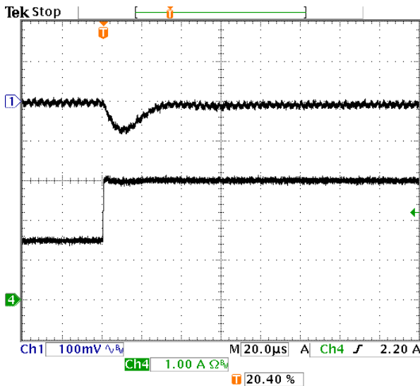
Fig-2.5V-6: Output voltage response for V_{out}=2.5V to positive load current step change from 1.5A to 3A with slew rate of 5A/\mu s at V_{in}=12V . C_o=47\mu F \times 2 ceramic.
