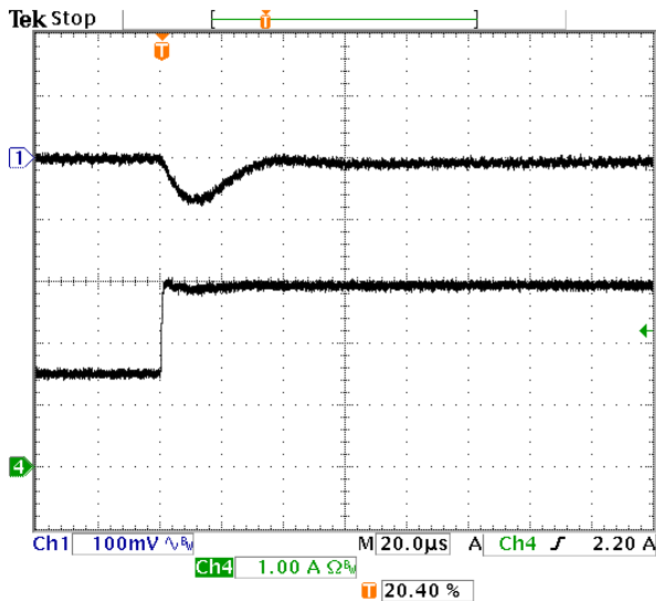
Fig-1.2V-6: Output voltage response for V_{out}=1.2V to positive load current step change from 1.5A to 3A with slew rate of 5A/\mu s at V_{in}=12V . C_o=47\mu F \times 2 ceramic.
