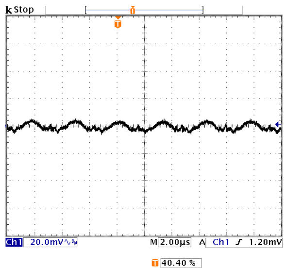
Fig-1.8V-5: Output voltage ripple (20mV/div.) for V_{out}=1.8V at full rated load current into a resistive load with external capacitance 47\mu F \times 2 ceramic + 1\mu F ceramic at V_{in}=12V . Time scale: 2 us/div
