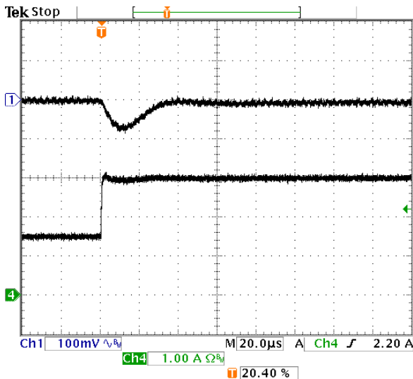
Fig-1.5V-6: Output voltage response for V_{out}=1.5V to positive load current step change from 1.5A to 3A with slew rate of 5A/us at V_{in}=12V . C_o=47\mu F \times 2 ceramic. Top trace: output voltage (100mV/div.) Bottom trace: load current (1A/div.) Time scale: 20us/div.
