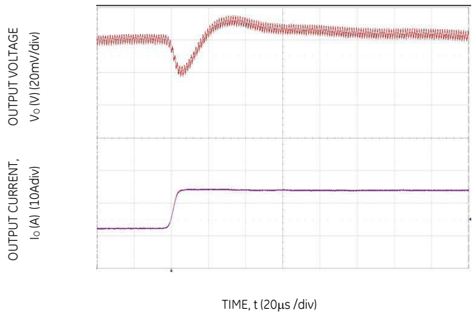
Figure 22. Transient Response to Dynamic Load Change from 50% to 100% at 12Vin, C_{out} = 2 \times 47 \mu F + 1 \times 330 \mu F , C_{Tune} = 3300 pF & R_{Tune} = 240 \Omega
