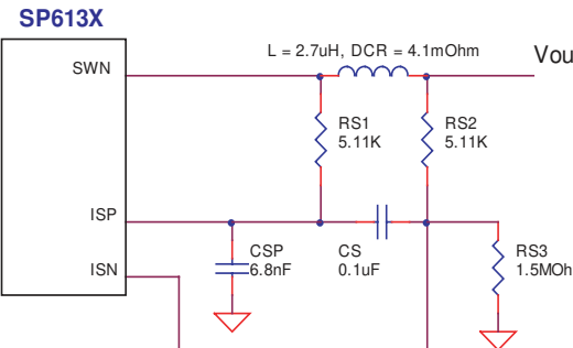
Figure 3- Over-current detection circuit for I_{MAX} < \{60mV / DCR\}
