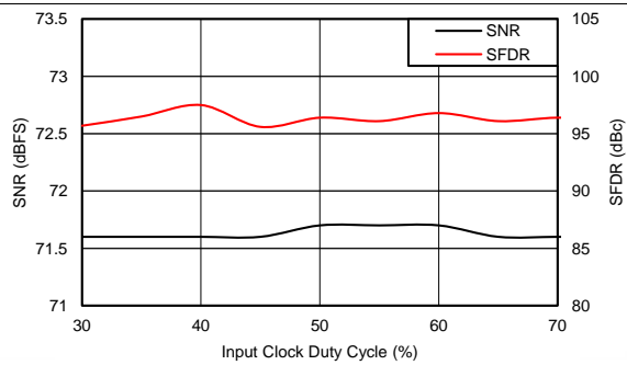
Figure 130. Performance vs Clock Duty Cycle (40 MHz)
