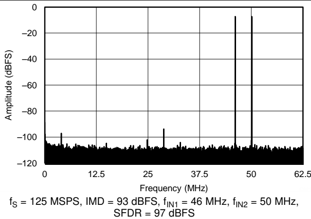
Figure 44. FFT for Two-Tone Input Signal (-7dBFS at 46 MHz and 50 MHz)
