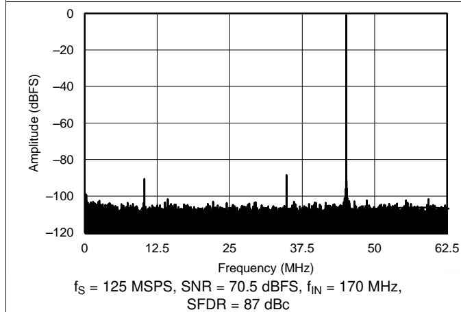
Figure 38. FFT for 170-MHz Input Signal, Dither On
