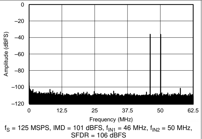
Figure 45. FFT for Two-Tone Input Signal (-36 dBFS at 46 MHz and 50 MHz)
