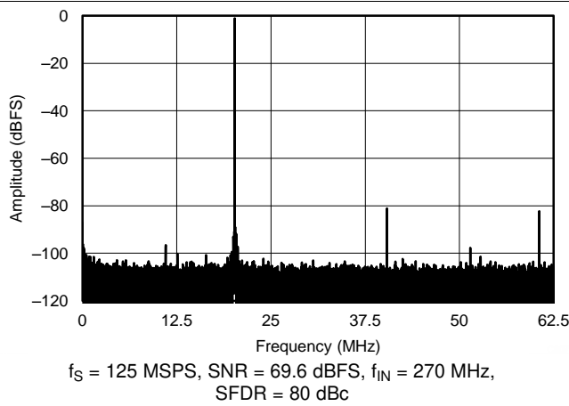
Figure 40. FFT for 270-MHz Input Signal, Dither On
