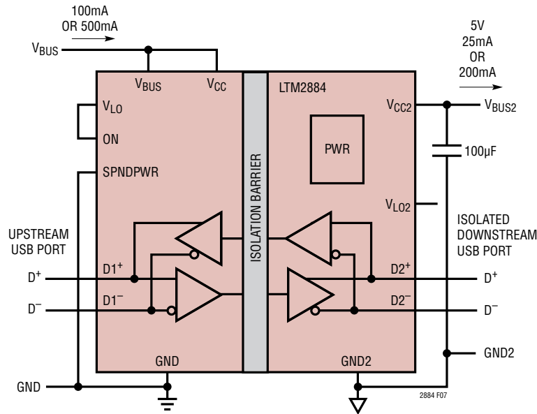
Figure 7. Bus Powered Inline Bus Splitter
