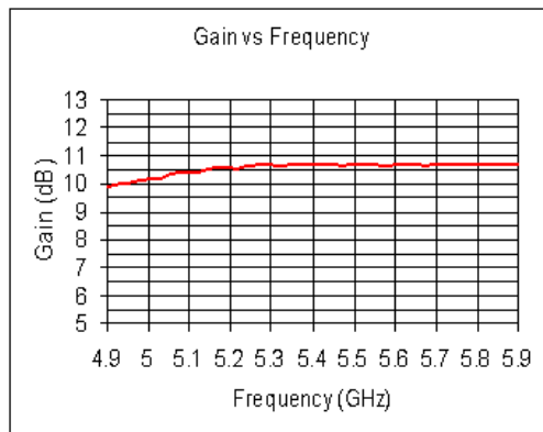
Figure 4 Gain Response
