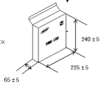
INNER BOX
