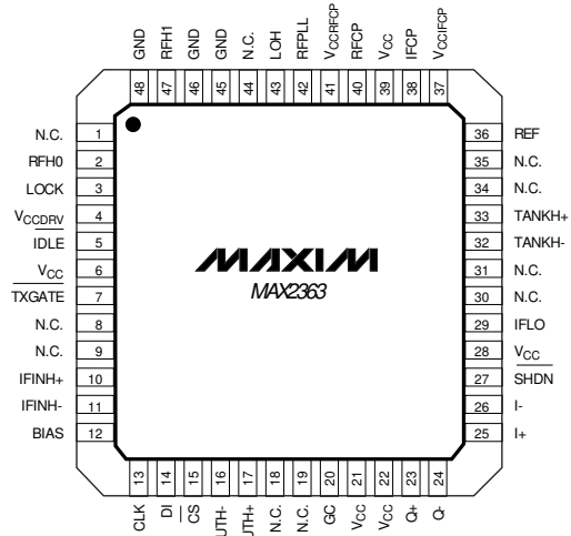
(T) QFN-EP
