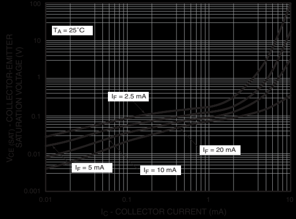
Figure 8. Collector-Emitter Saturation Voltage vs. Collector Current
