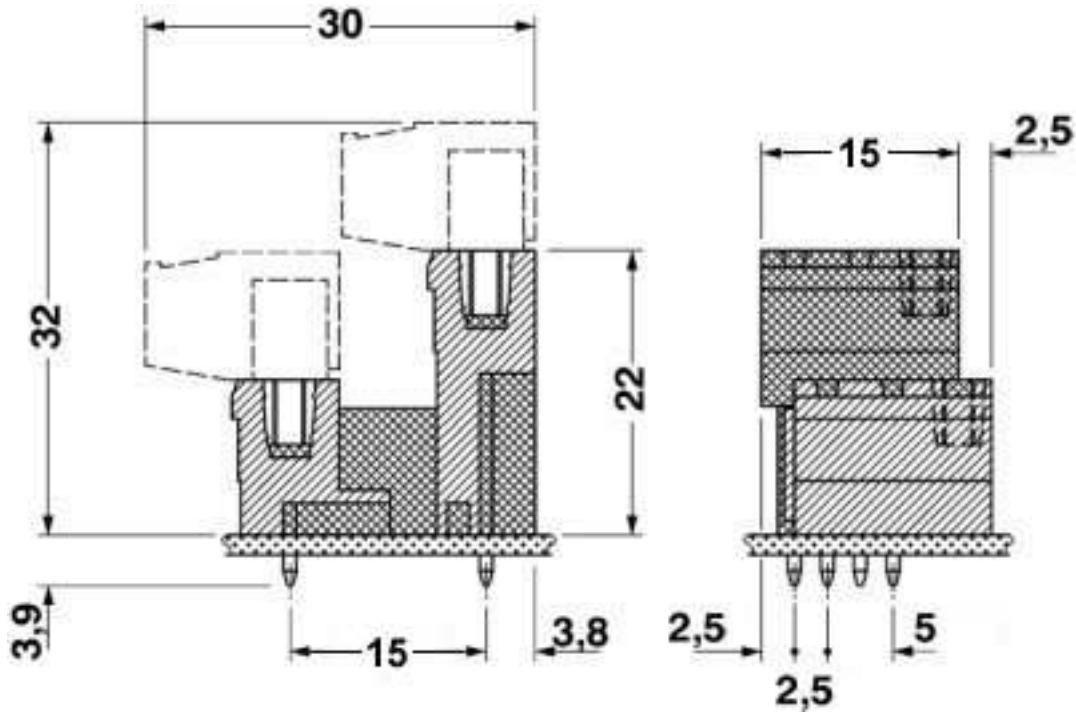
Dimensioned drawing
