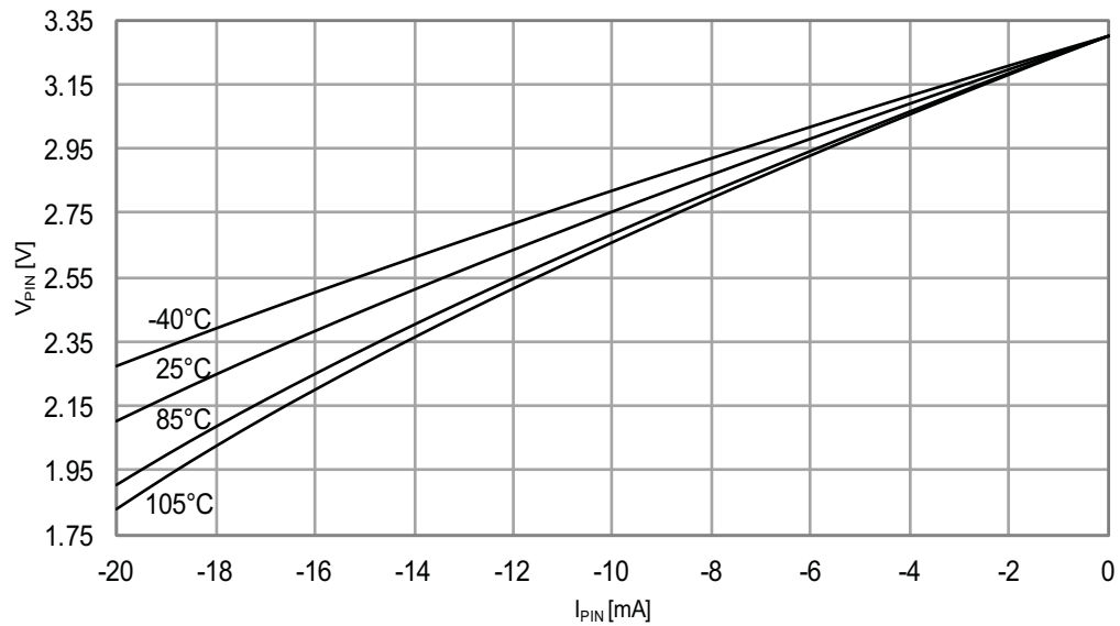
Figure 37-22. I/O Pin Output Voltage vs. Source Current
