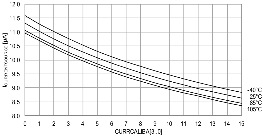
Figure 37-49. Analog Comparator Current Source vs. Calibration
