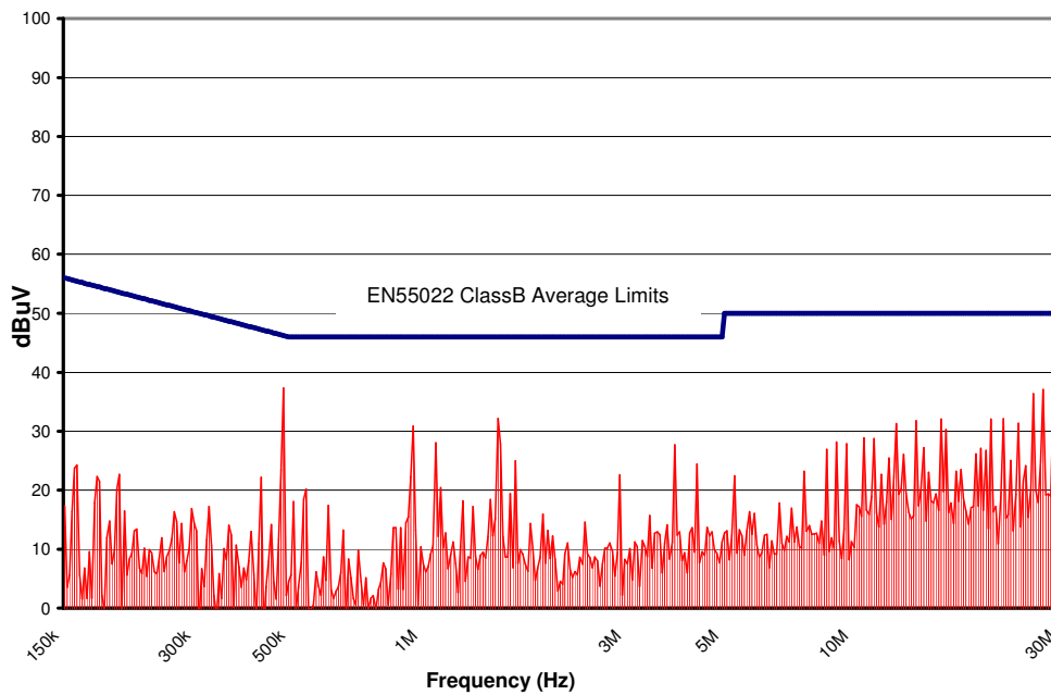
Figure 19. CPT15F36N Conducted Emissions using above specified input filter. Vin = 48V, Full Resistive Load
