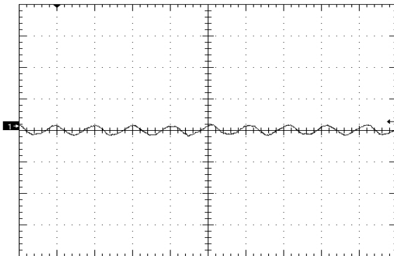
Figure 9. Input Reflected Ripple Current (5mA/div) time scale - 2uS/div. Vin=Vin_nom, full resistive
