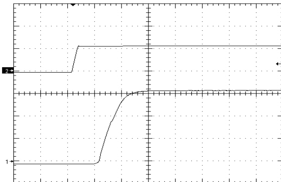
Figure 11. Waveform (1V/div) via Line Voltage, time scale 10mS/div. Vin=24Vin, full resistive load + 10000uF across output.
