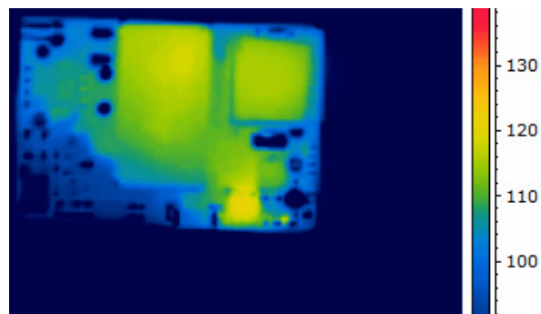
Figure 6. Thermal Image of CPT15F36 (15A output, 70C Ambient, 200lfm airflow, Vin = 48V, airflow from pin 3 to pin 1, T max = 122°C)
