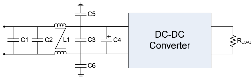
Figure 18. EMI Filter
