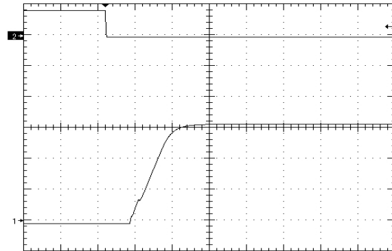
Figure 10. Startup Waveform (1V/div) via Enable Pin, time scale 10mS/div. Vin=Vin_nom, full resistive load + 10000uF (negative enable.)
