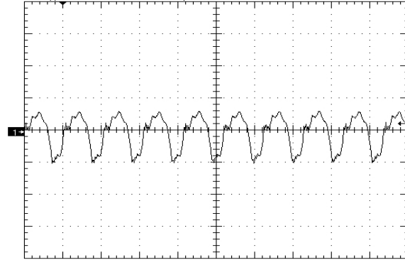
Figure 8. Output Voltage Ripple (20mV/div), time scale - 2uS/div. Vin=Vin_nom, full resistive Cout=1uF ceramic + 100uF Tantalum (see Fig 15)
