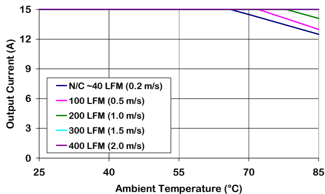
Figure 4. Output Current Derating vs Ambient Temperature & Airflow (converter mounted vertically with air flowing from pin 3 to pin 1, Vin = 24 V.)
