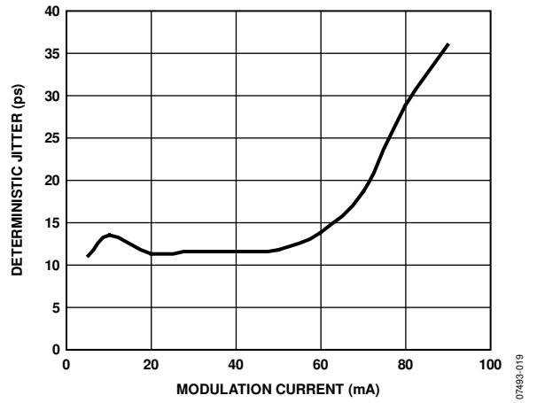
Figure 14. Deterministic Jitter at 4.25 Gbps vs. Modulation Current, I_{BIAS} = 20 mA
