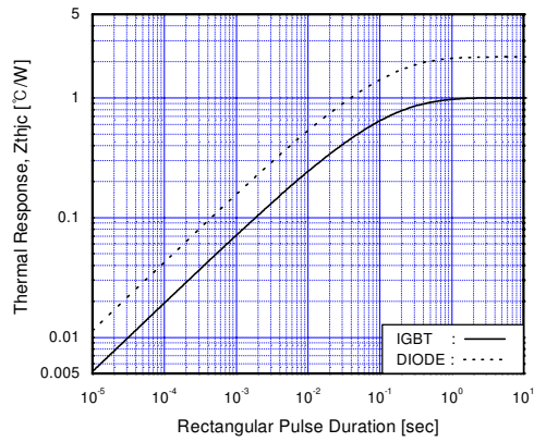
Fig 18. Transient Thermal Impedance
