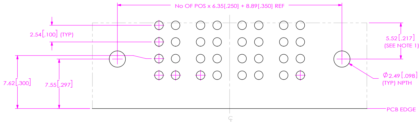
FIG 2 PCB LAYOUT FOR PET-XX-XX-XX-RA-LC SHOWN (SAME AS FIG 1, UNLESS OTHERWISE STATED)
