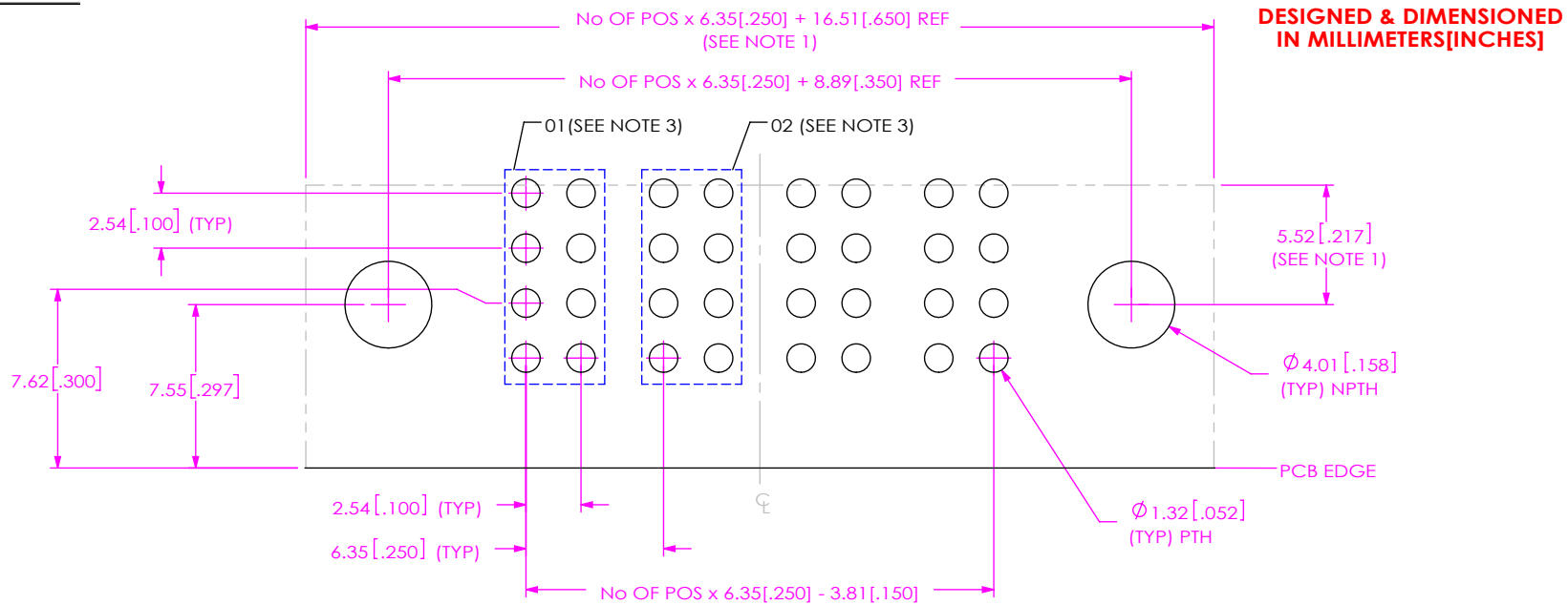
FIG 1 PCB LAYOUT FOR PET-XX-XX-XX-RA-SD SHOWN
