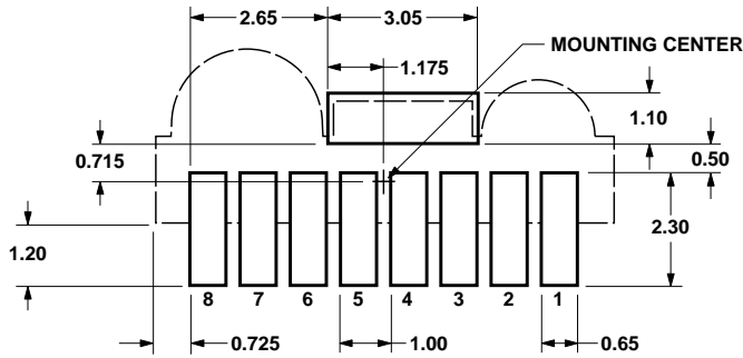
Figure 17. Land pattern.
