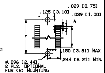
CONNECTOR SIDE
