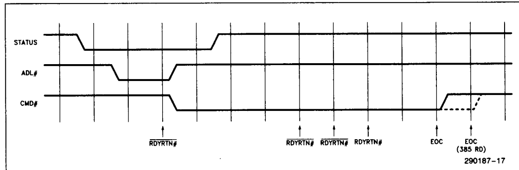
Asynchronous Extended
