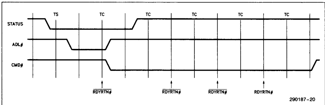
Asynchronous Extended
