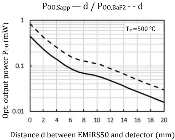
Optical output power ( P_{OO} ) versus distance d of a 1 mm 2 detection surface at 500°C T_M
