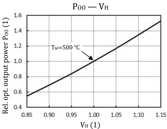
Relative change of optical output power ( P_{OO} ) by changing heater voltage ( V_H )
