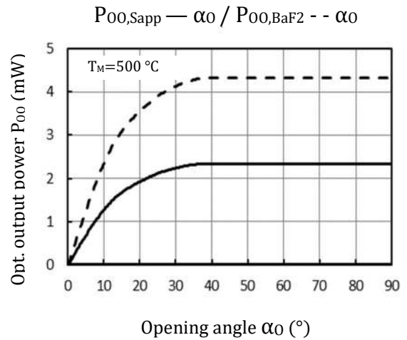
Optical output power ( P_{OO} ) versus opening angle \alpha_0 (integral rotation of a cone) at 500°C T_M
