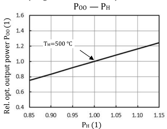
Relative change of optical output power ( P_{OO} ) by changing heater power ( P_H )
