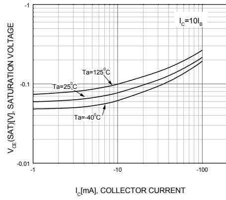
Figure 2. Collector-Emitter Saturation Voltage
