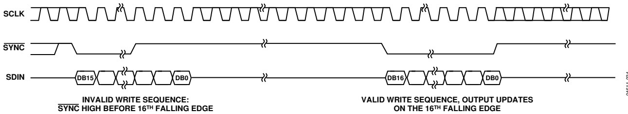
Figure 36. SYNC Interrupt Facility
