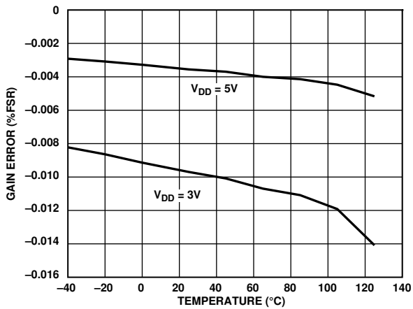
Figure 18. Gain Error vs. Temperature (3 V/5 V)
