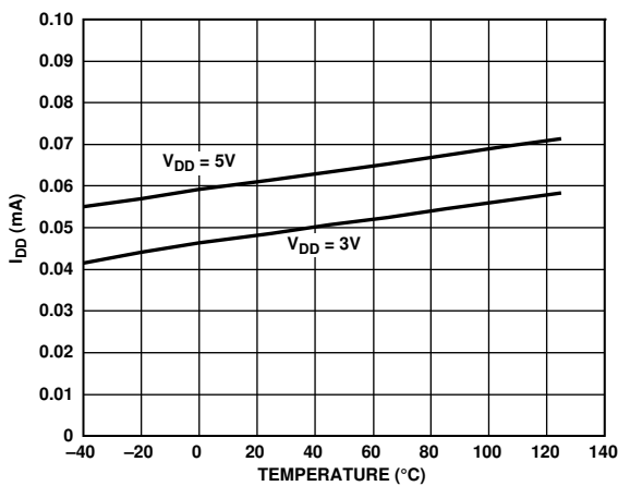
Figure 19. Supply Current vs. Temperature (3 V/5 V Supply)
