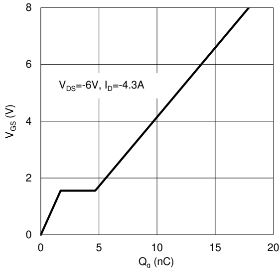
Figure 23. Gate Charge
