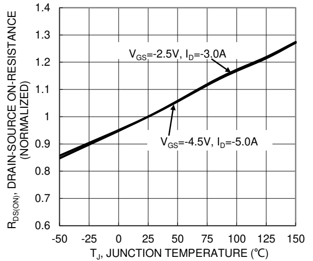
Figure 18. On-Resistance Variation with Temperature
