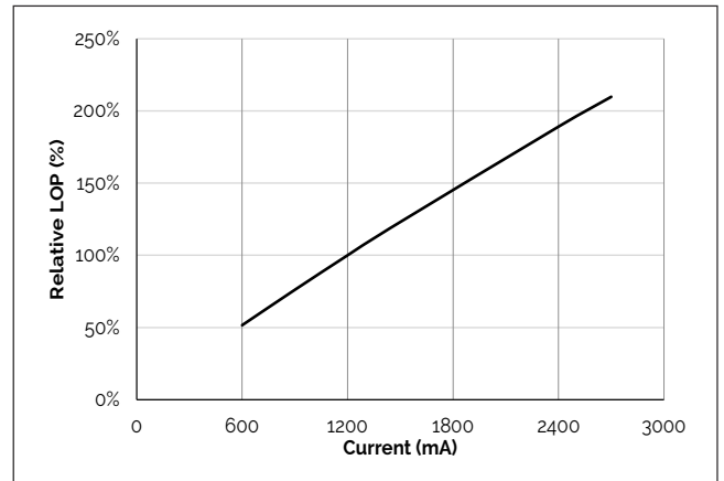
Figure 4: V22C Typical Relative Flux vs. Current
