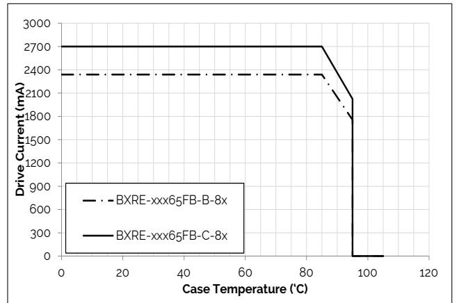
Figure 6: Derating Curve
