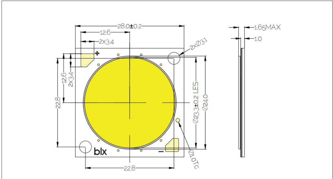
Figure 10: Drawing for V22 LED Array
