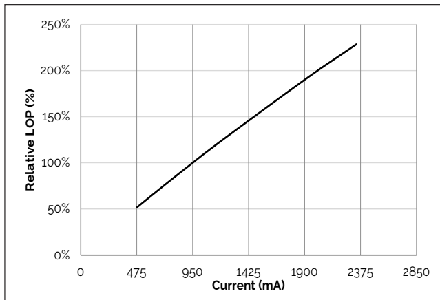
Figure 3: V22B Typical Relative Flux vs. Current
