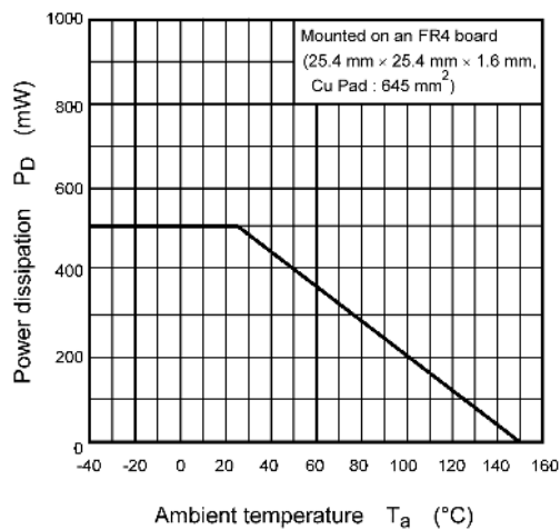
Fig. 8.13 P_D - T_a
