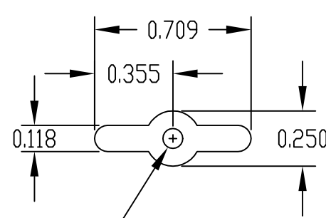
DETAIL "C" (4) PLACES
