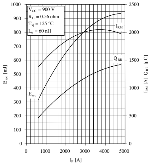
Fig. 13 Typical reverse recovery characteristics vs forward current
