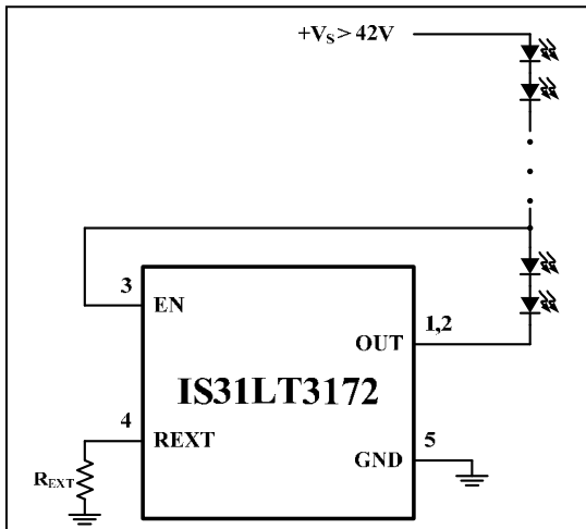
Figure 38 High Input Voltage Application Circuit
