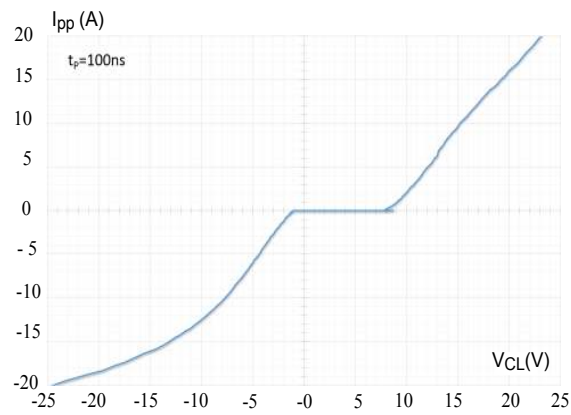
Figure 16. TLP characteristic
