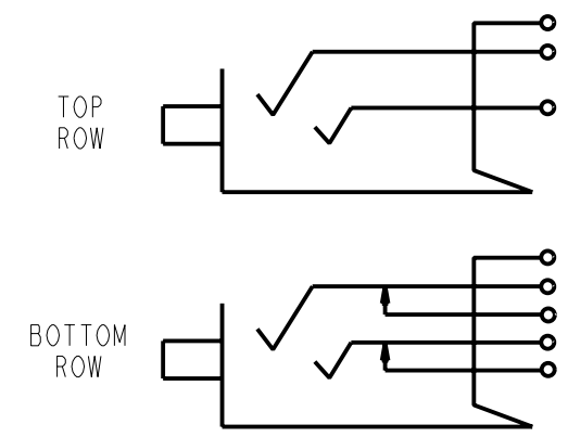
IT JACK SCHEMATIC
