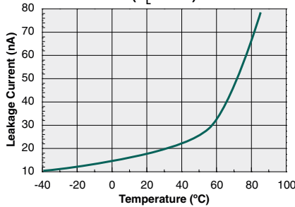
Typical Leakage Current vs. Temperature ( V_L=800\text{V} )
