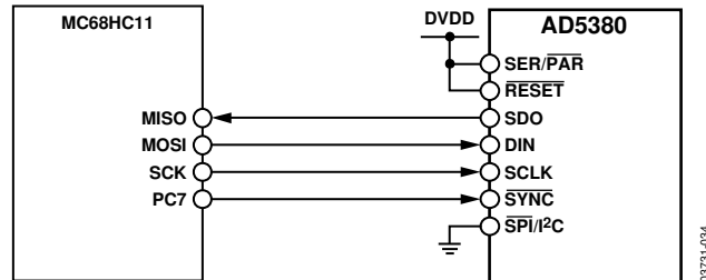
Figure 34. AD5380-to-MC68HC11 Interface
