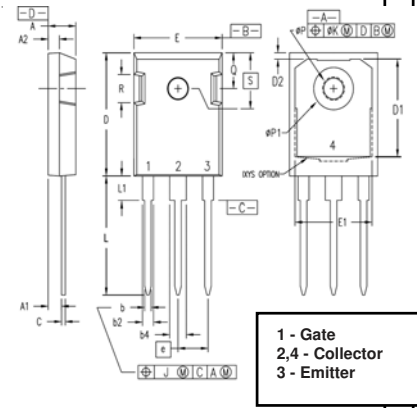
TO-247 (IXXH) Outline
