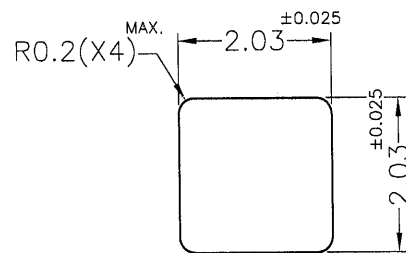
MOUNTING HOLE
