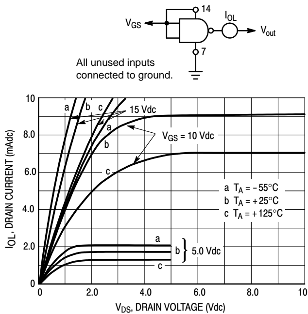
Figure 4. Typical Output Sink Characteristics Test Circuit
